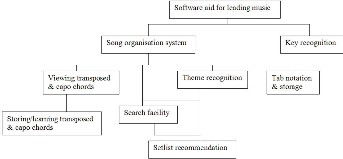
Figure 2: The dependencies and relationships between the key features of the software part of the project. This shows what tasks can be done in parallel and in what order, with tasks at the top needing to be done first.
