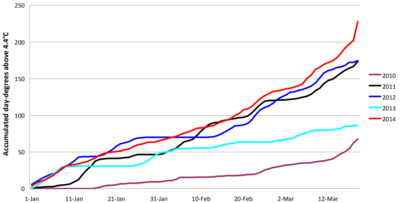
Accumulated day-degrees at Wellesbourne (above 4.4°C) from 1 January in 2010-2014
