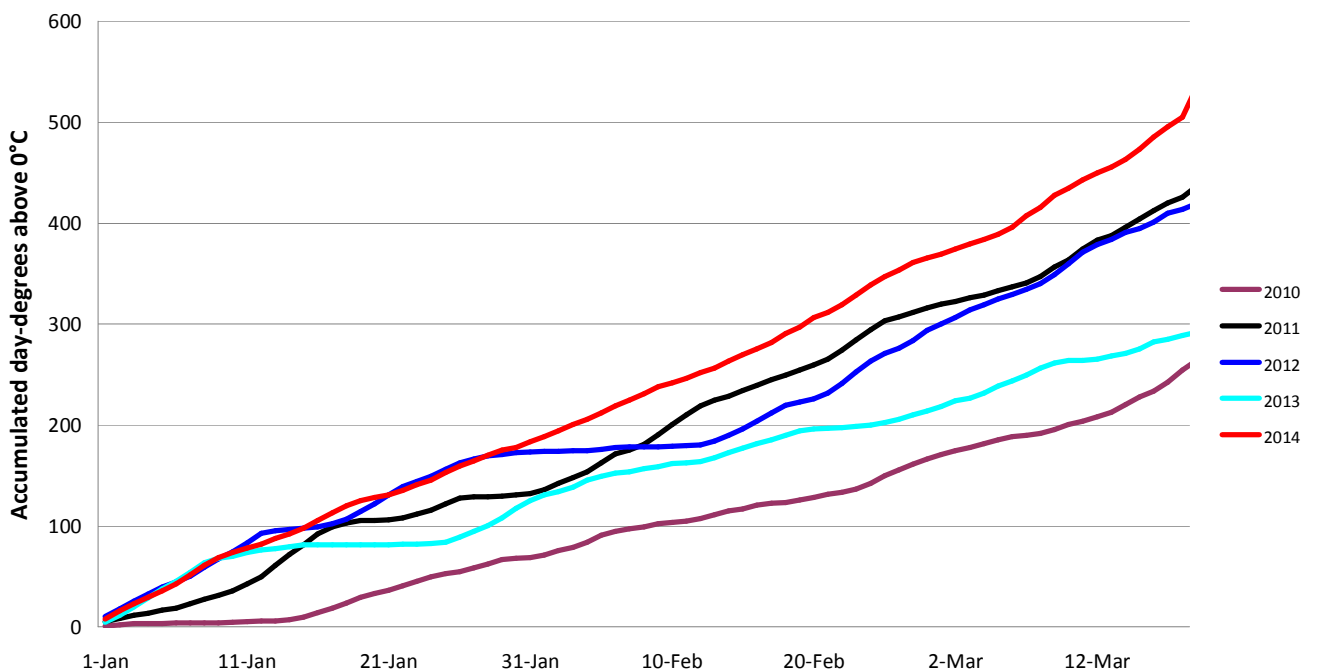
Accumulated day-degrees at Wellesbourne (above 0°C) from 1 January in 2010-2014
